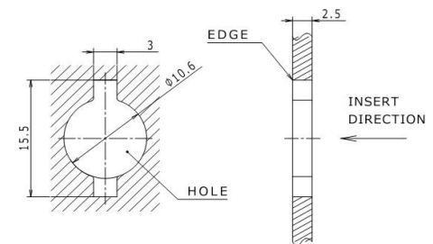
FITTING HOLE SHAPE (REFERENCE)
